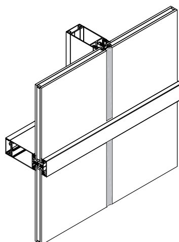
MATRIX Msg (semi structural glazing)
