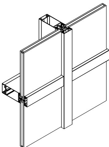
MATRIX Mrg (regular glazing)
