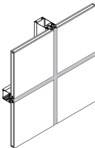
MATRIX Msg (structural glazing)
